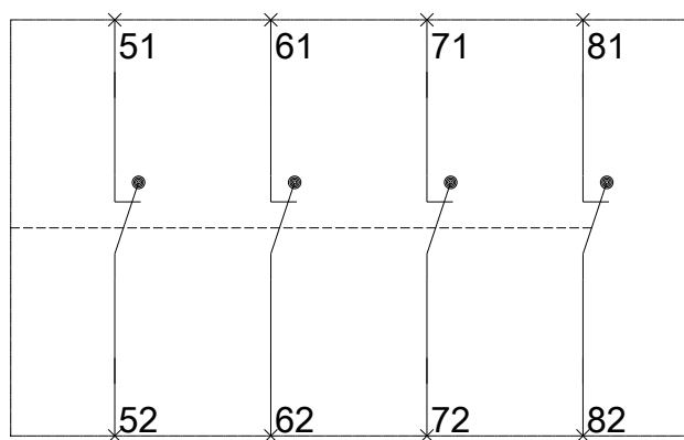
3RT2
