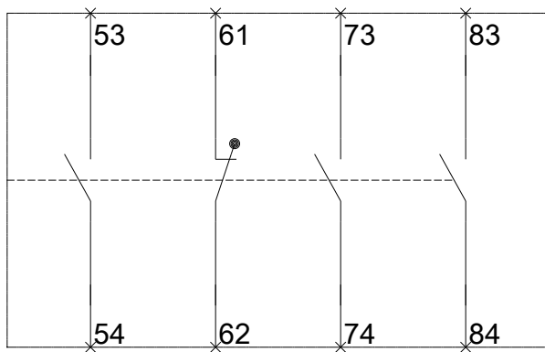
3RT2
