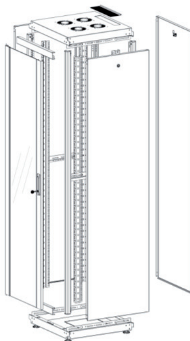
EXPLODED VIEW
