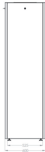
REAR VIEW
